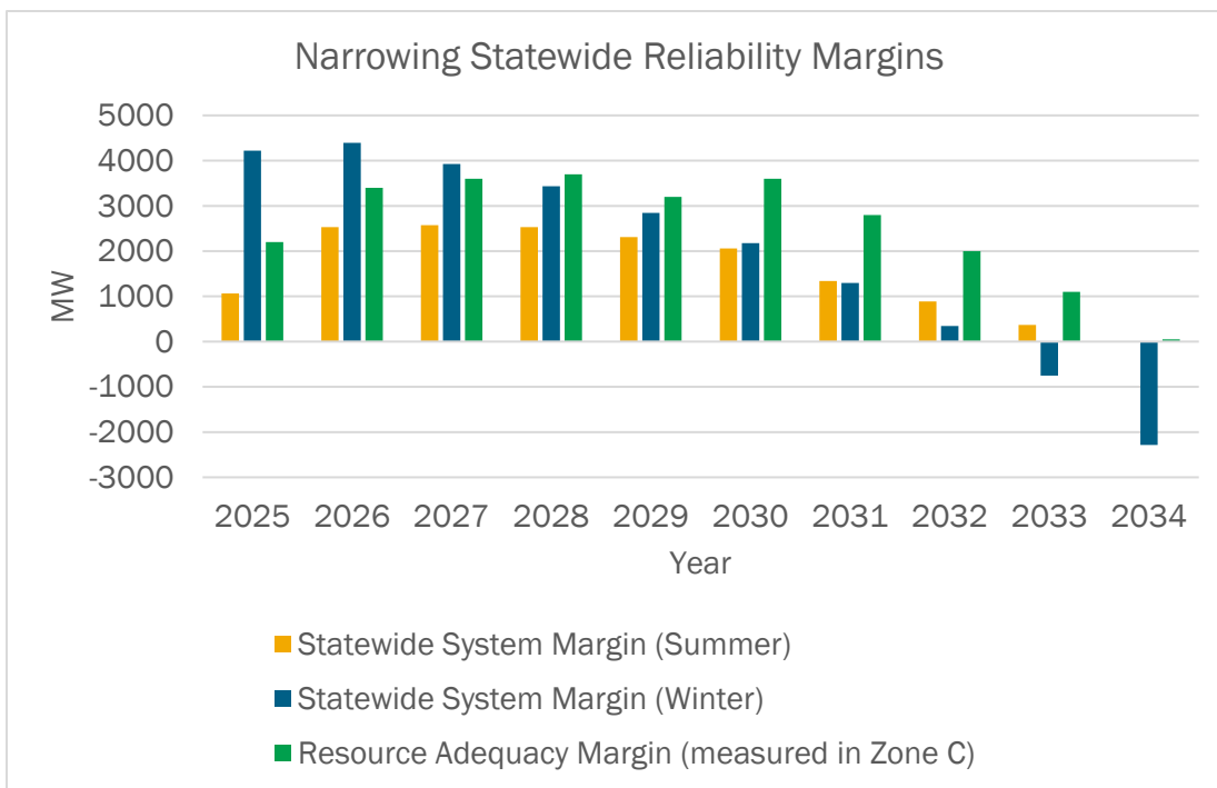
Figure 4: Narrowing Statewide Reliability Margins
