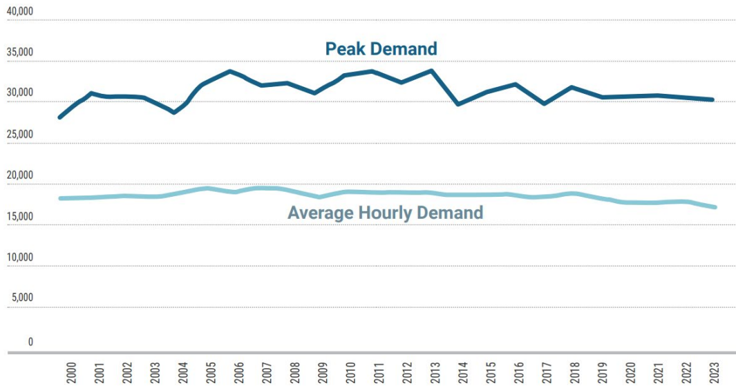
Figure 11: Historical Average Hourly Demand versus Actual Yearly Summer Peak Demand
