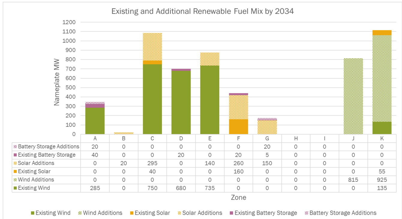
Figure 21: Existing and Additional Renewable Fuel Mix by 2034 - MW
