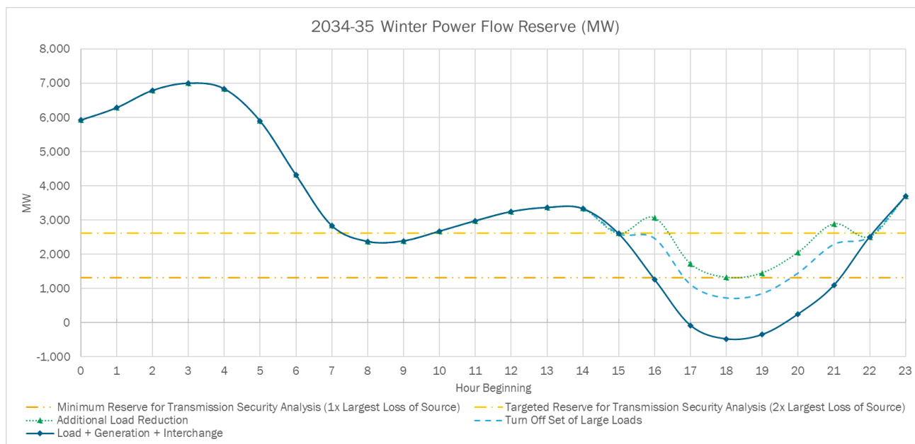
Figure 29: 2034-2035 Winter Peak Day Reserve Levels
