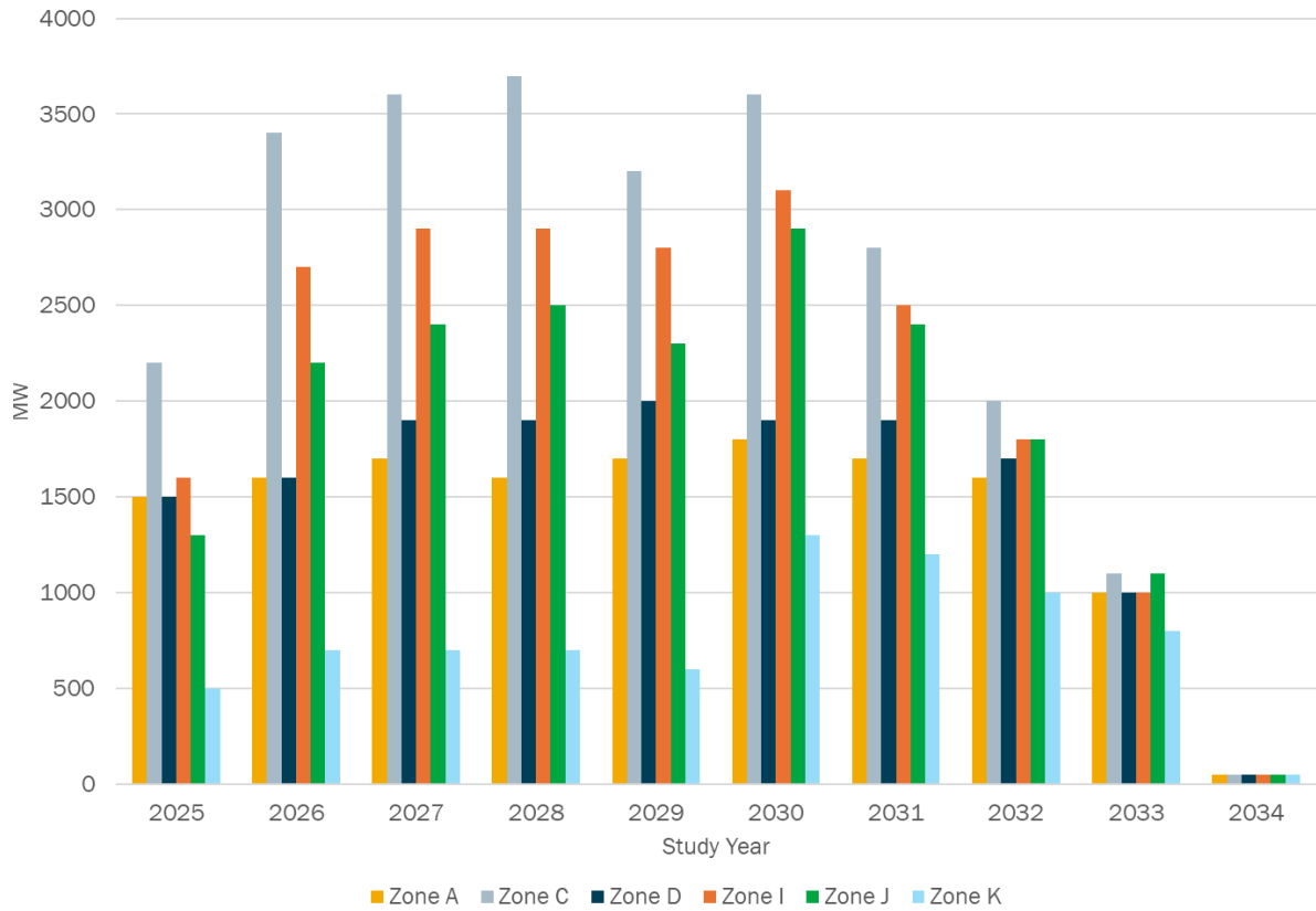
Figure 26: Zonal Resource Adequacy Margins - ZRAM (MW)
