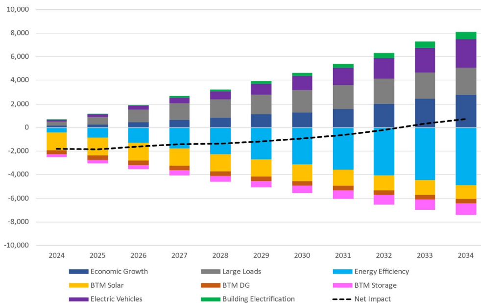
Figure 15: NYCA Baseline Summer & Winter Peak Forecast Impacts - MW
