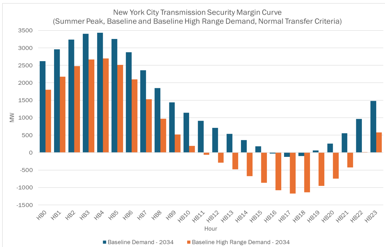
Figure 33: New York City Transmission Security Margin Hourly Curve - 2034
