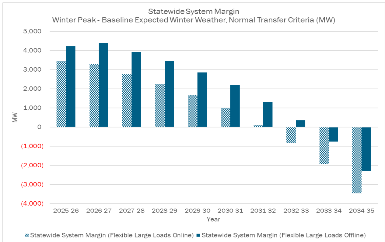
Figure 28: Winter Peak Statewide System Margin
