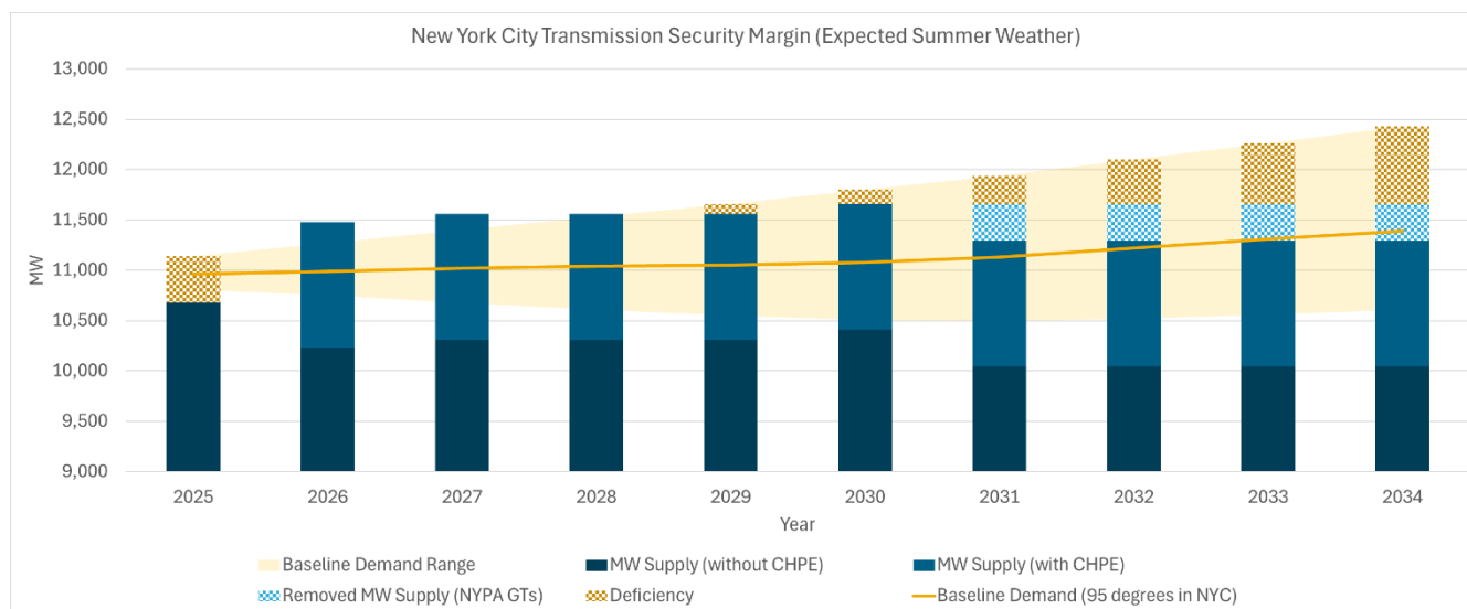
Figure 1: New York City Margin Forecast Uncertainty
