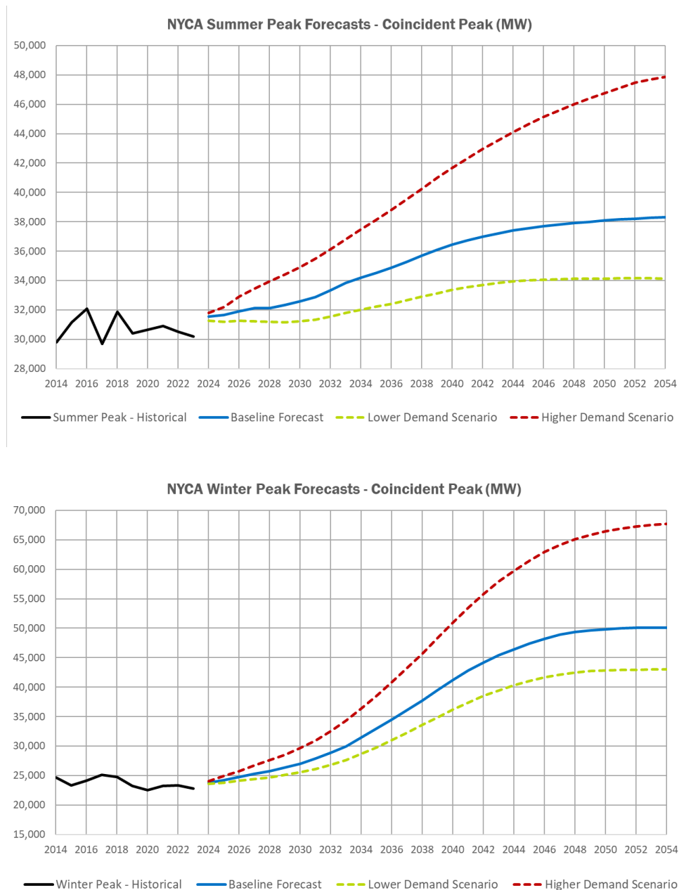
Figure 14: 30-Year NYCA Summer and Winter Peak Forecasts
