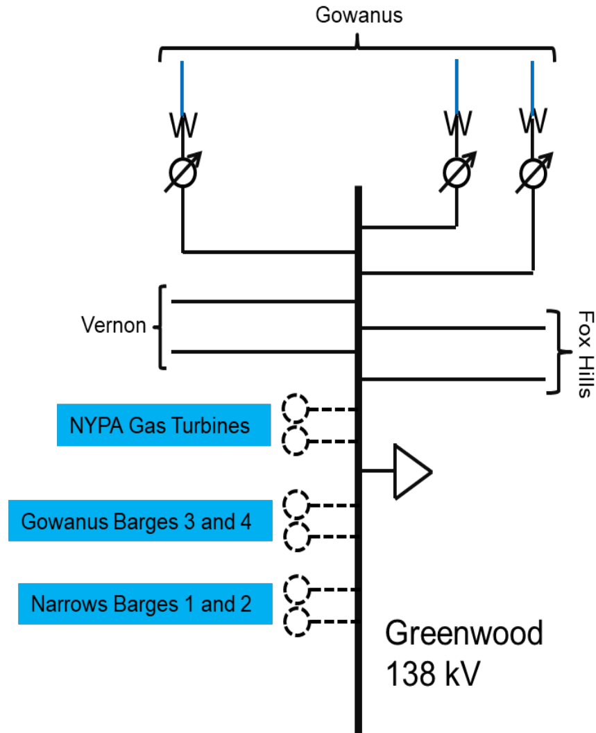
Figure 34: Greenwood 138 kV TLA
