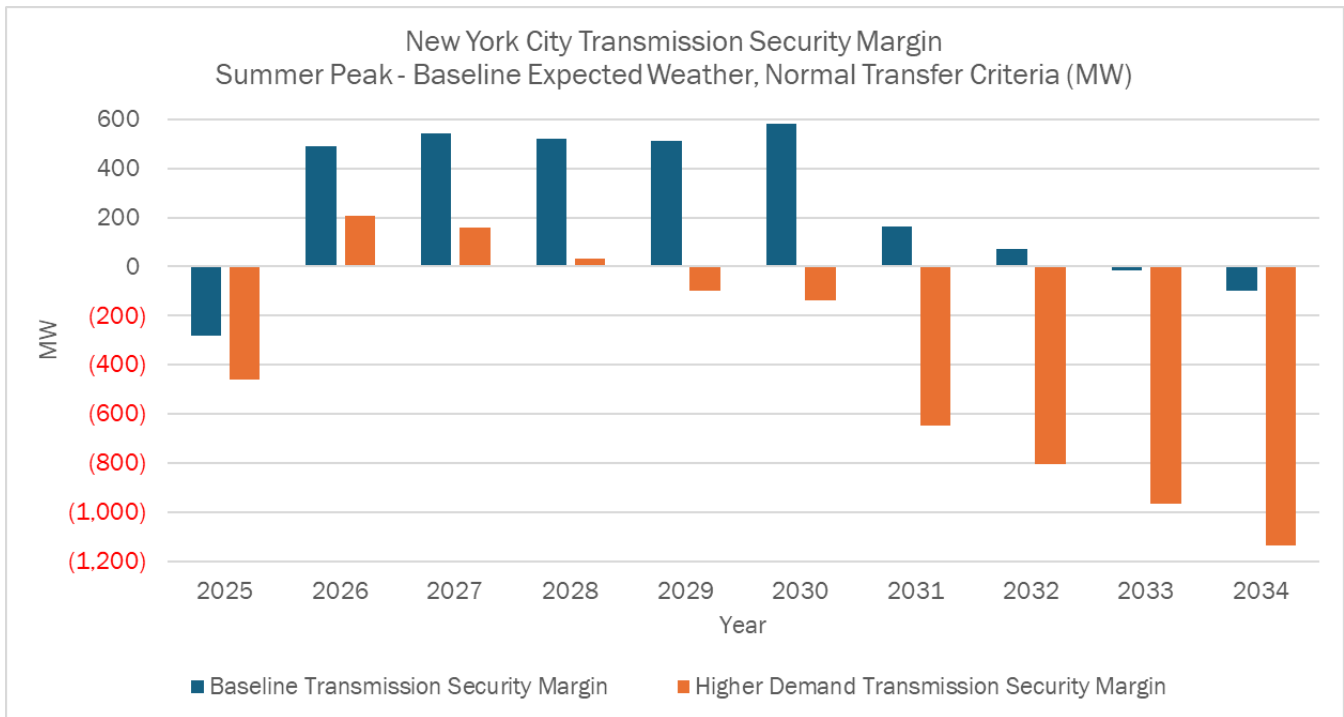
Figure 32: New York City Transmission Security Margin
