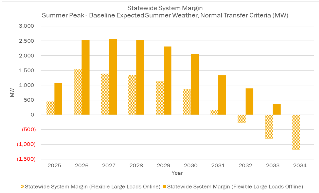
Figure 27: Summer Peak Statewide System Margin
