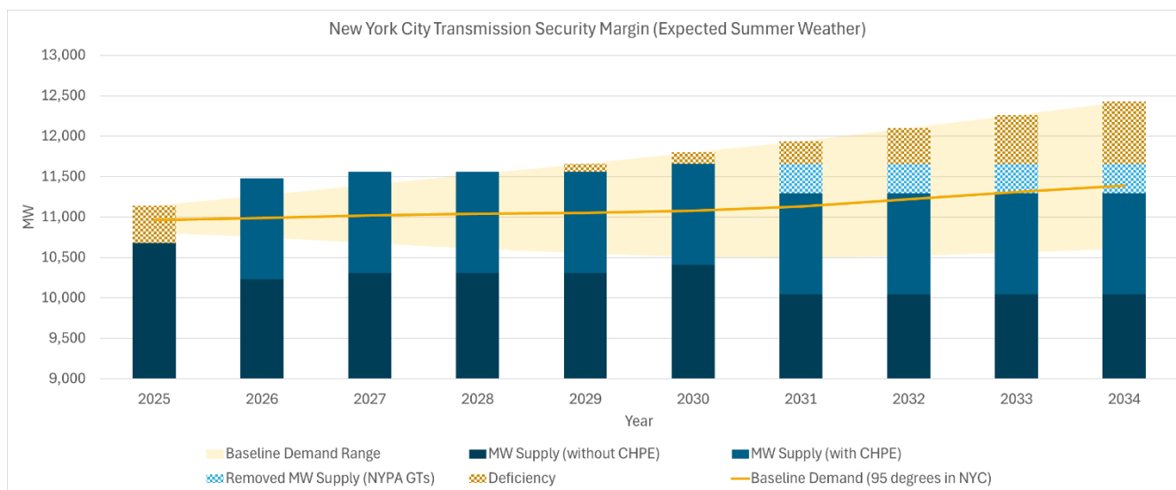
Figure 44: New York City Margin Forecast Uncertainty
